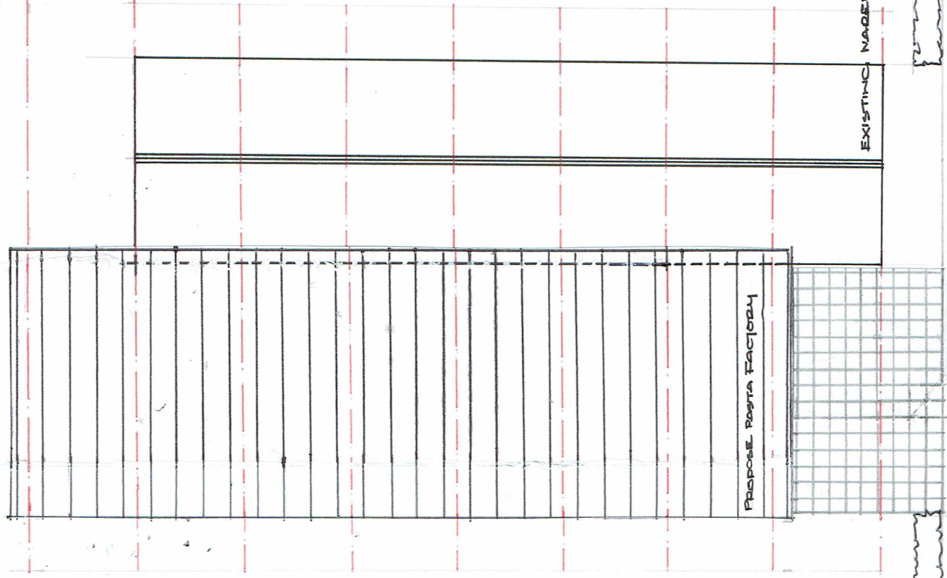
ROOF PLAN AS PROPOSED SCALE 1:200 @ A3
